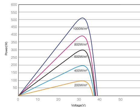
P-V CURVES OF PV MODULE(510W)
