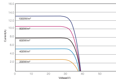
I-V CURVES OF PV MODULE(510W)
